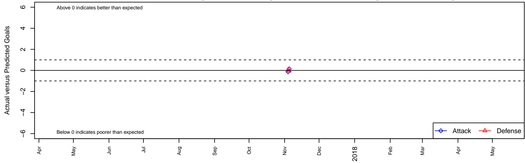
Pateadores Academy USSDA B04 Dots are actual minus expected GF (blue circles) and GA (red triangles). Blue line is smoothed change in attack strength. Red is smoothed change in defense strength.
